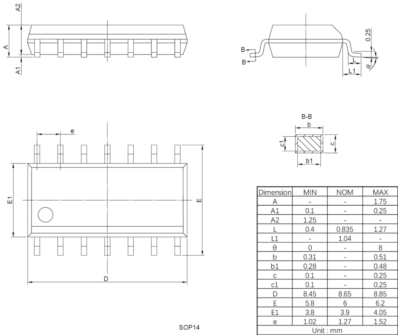
Figure 6. SOP14 Outline Dimensions
