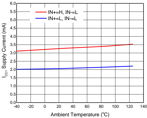
Figure 14. I_{CC1} Supply Current vs Temperature
