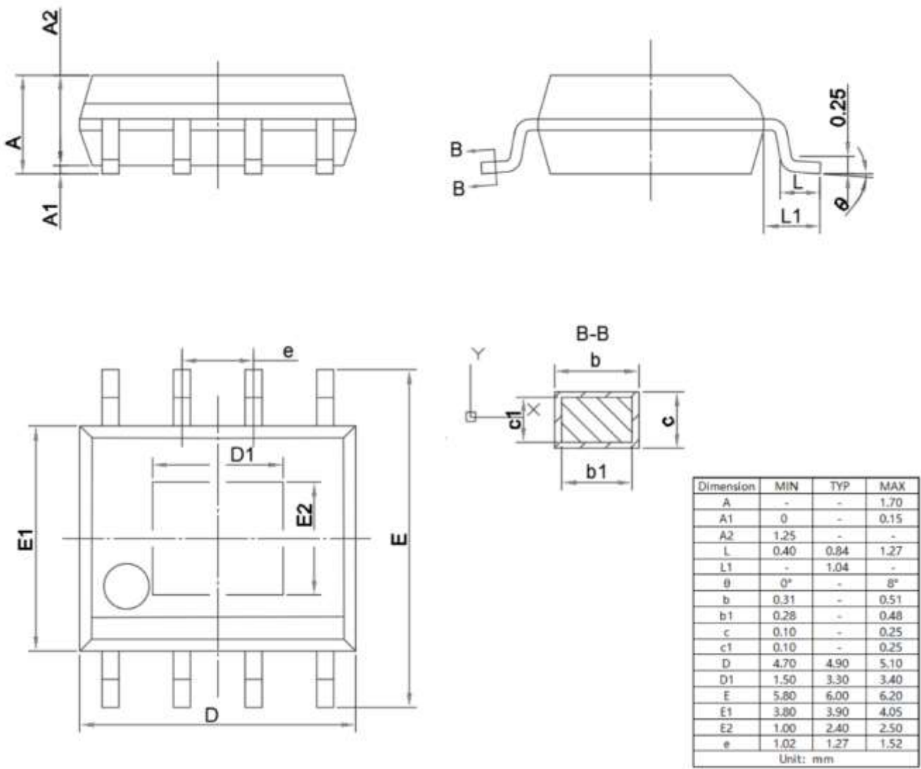
Figure 23. SOP8-EP Outline Dimensions
