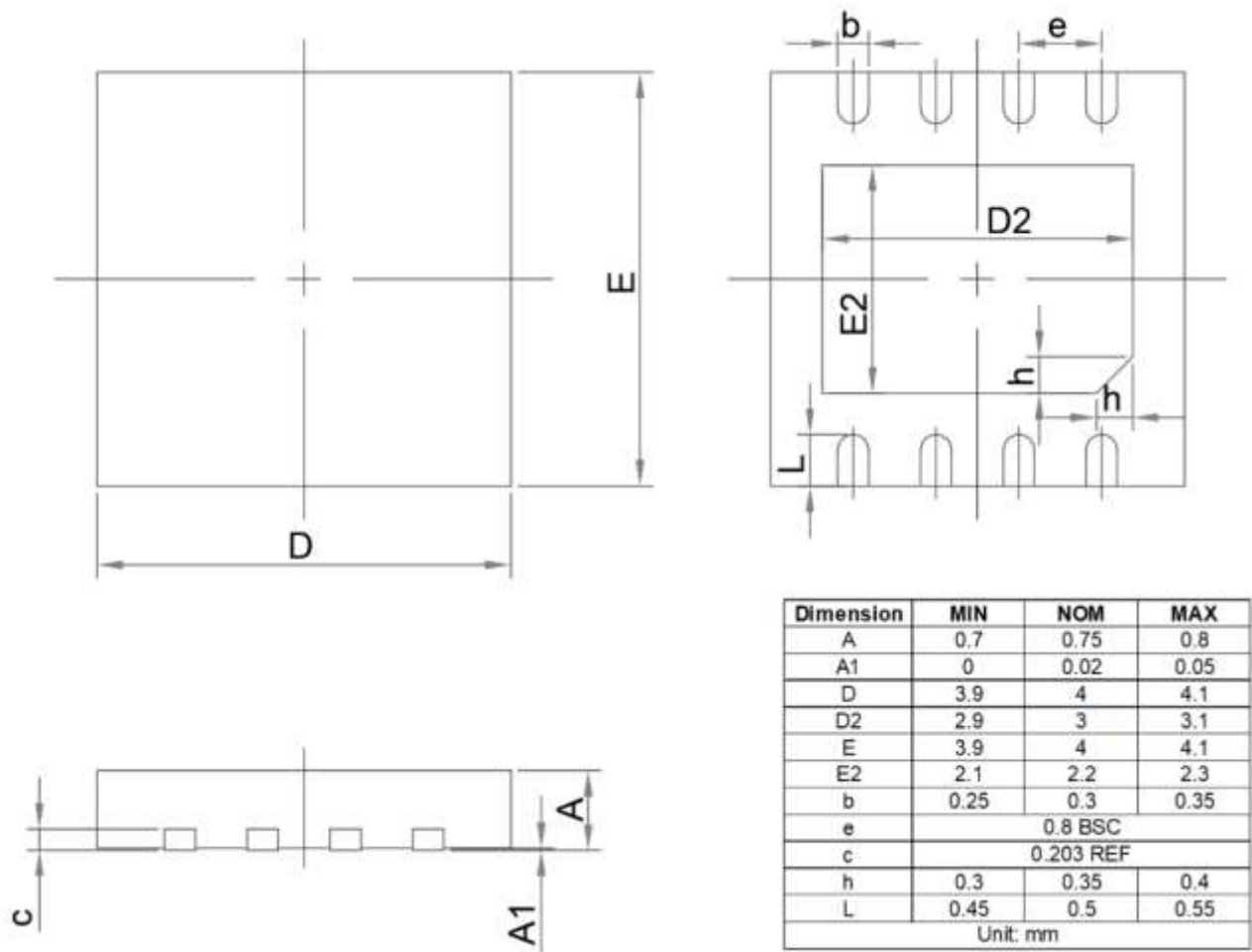
Figure 24. DFN4x4-8 Outline Dimensions
