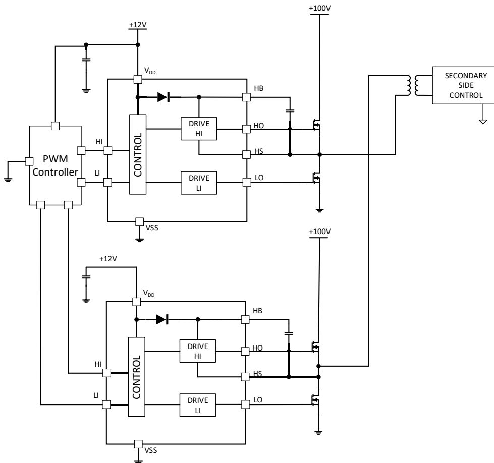
Figure 21. SLM27211 Typical Application Circuit in Full Bridge
