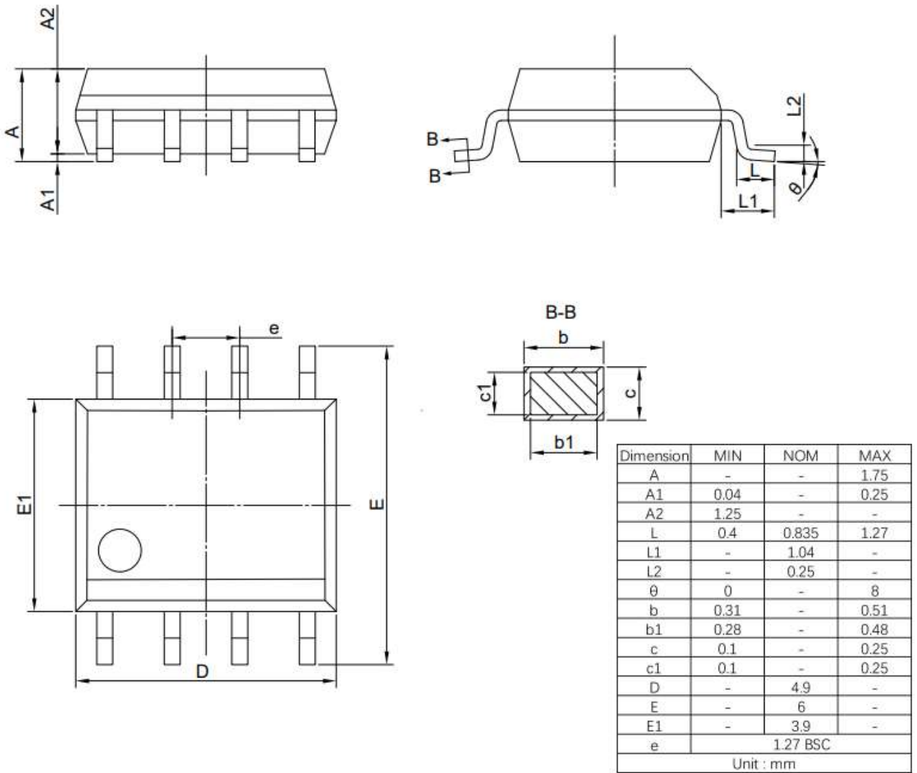
Figure 22. SOP8 Outline Dimensions
