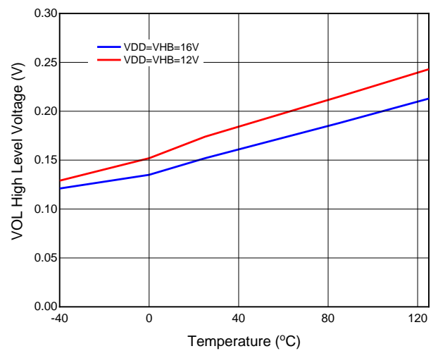
Figure 13. LO High Level Output Voltage vs Temperature
