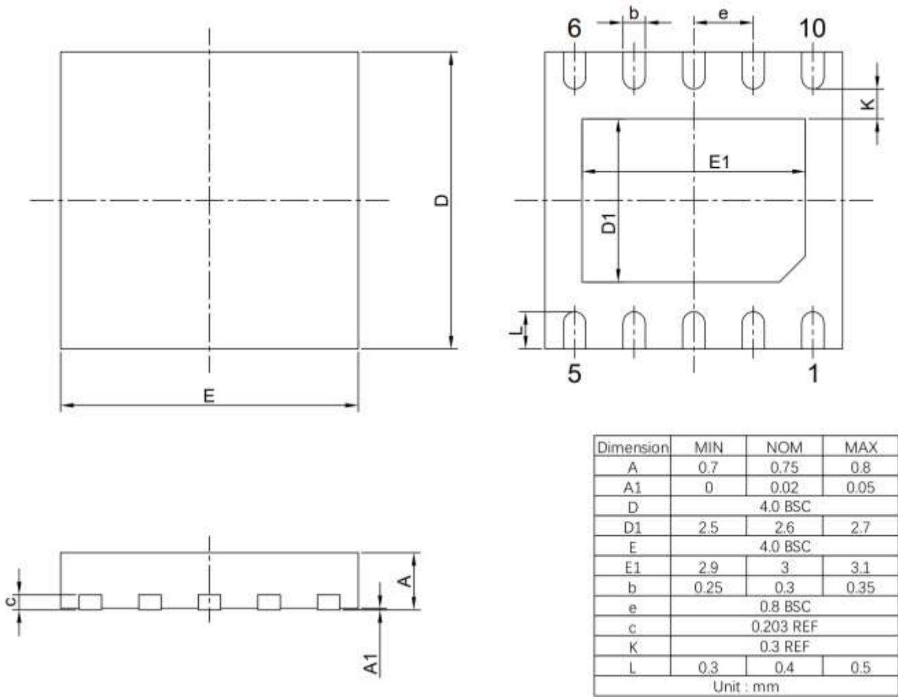
Figure 25. DFN4x4-10 Outline Dimensions
