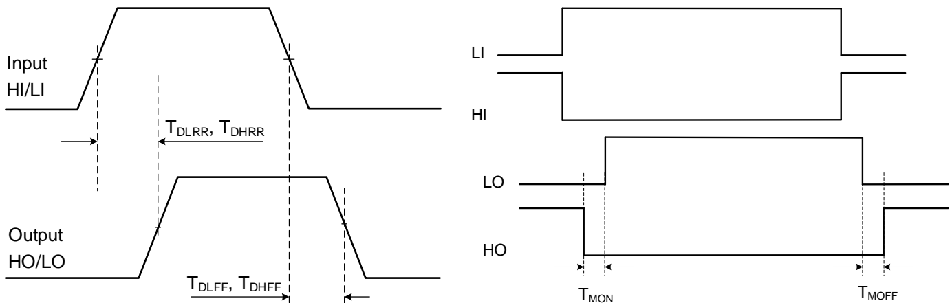
Figure 1. Timing Diagram
